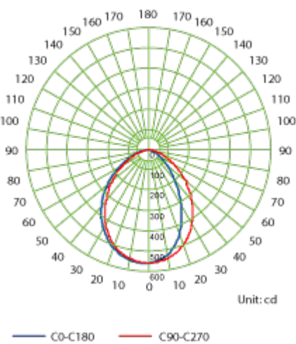
Luminous Intensity Distribution Curve - 4008.204.104
