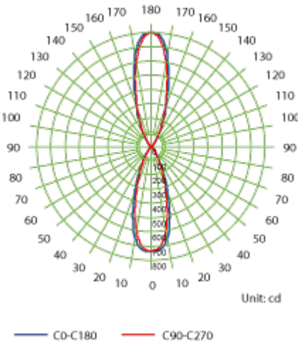
Luminous Intensity Distribution Curve - 4009.205.1XL
