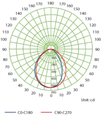
Luminous Intensity Distribution Curve - 4005.204.104
