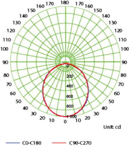
Luminous Intensity Distribution Curve - 4520.141.104
