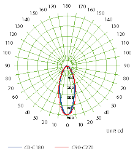
Luminous Intensity Distribution Curve - 2061.100.7T4
