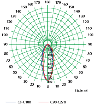
Luminous Intensity Distribution Curve - 5080.105.1XL
