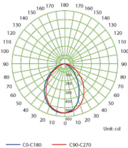
Luminous Intensity Distribution Curve - 4005.204.104
