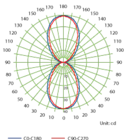
Luminous Intensity Distribution Curve - 4009.102.1F5
