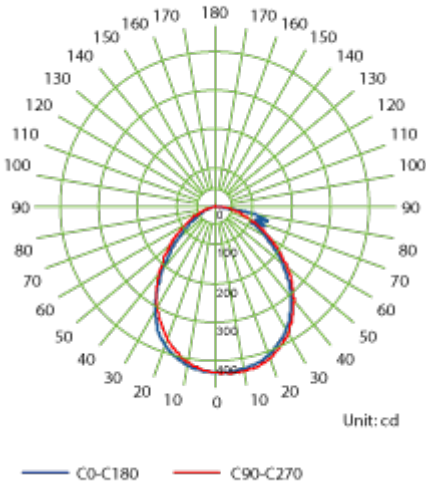
Luminous Intensity Distribution Curve - 4007.204.204
