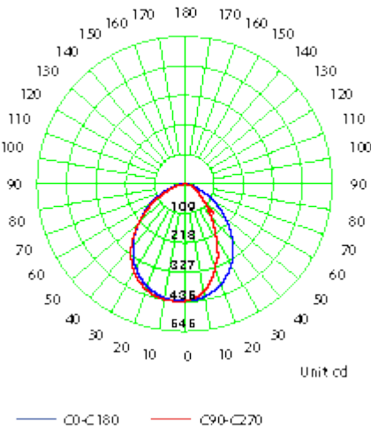
Luminous Intensity Distribution Curve - 4002.104.104
