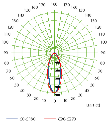
Luminous Intensity Distribution Curve - 2061.100.2F4
