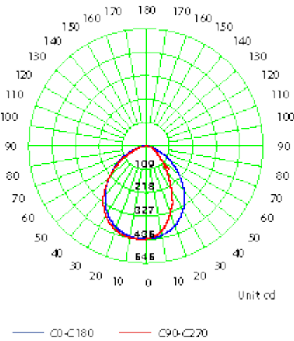
Luminous Intensity Distribution Curve - 4002.104.704
