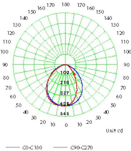
Luminous Intensity Distribution Curve - 4002.204.104
