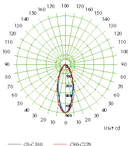
Luminous Intensity Distribution Curve - 2061.100.2T4
