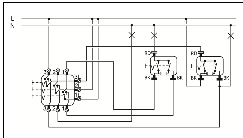
Wiring diagram 5306 EU
