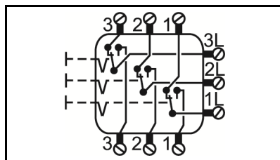
Contact assignments
