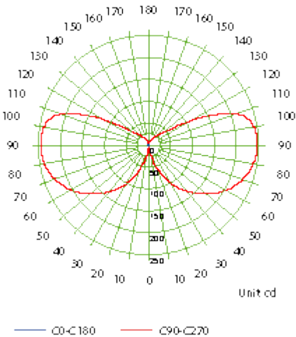
Luminous Intensity Distribution Curve - 4004.204.1 F4
